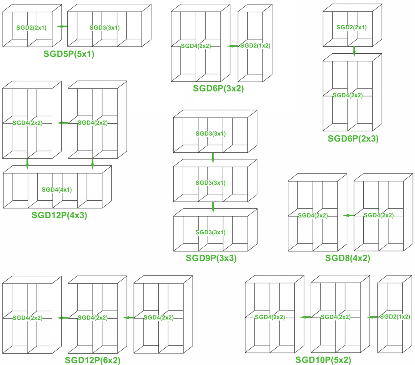
Diagram 2: The Larger size dispensers (below) are made up of packages of the core product range (above)
