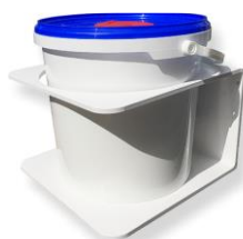
WTH-215. Wipes Tub/Bucket Holder for Clinical & Industrial types. Wall Mounting
